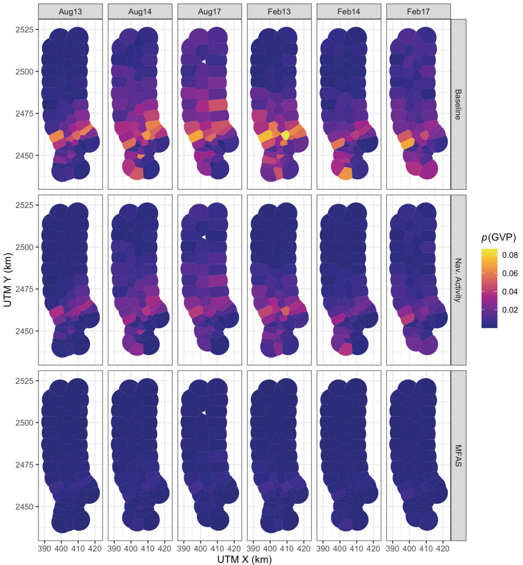
FIGURE 3 Map of expected probability of detecting a group vocal period (GVP; color scale) at each hydrophone during each Submarine Commander Course (SCC; columns) prior to the onset of naval training activity, during naval training activity when no mid-frequency active sonar (MFAS) was present, and during naval training activity when MFAS was present at a received level of 150 dB re 1 \mu\text{Pa} rms (rows).
